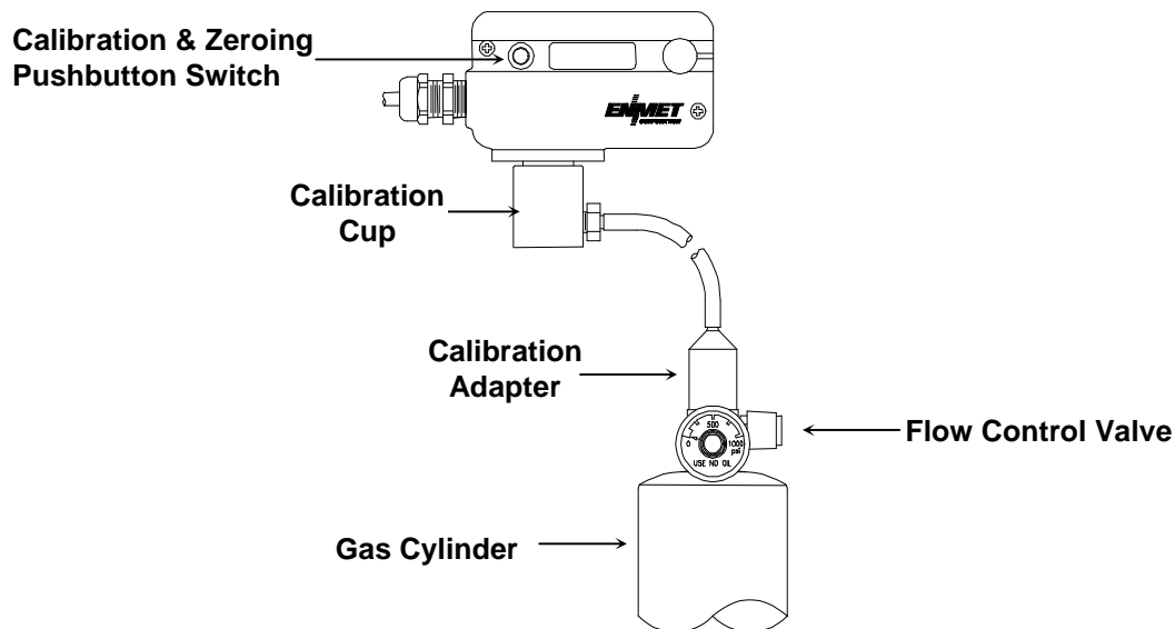
Figure E: Calibration with Gas
