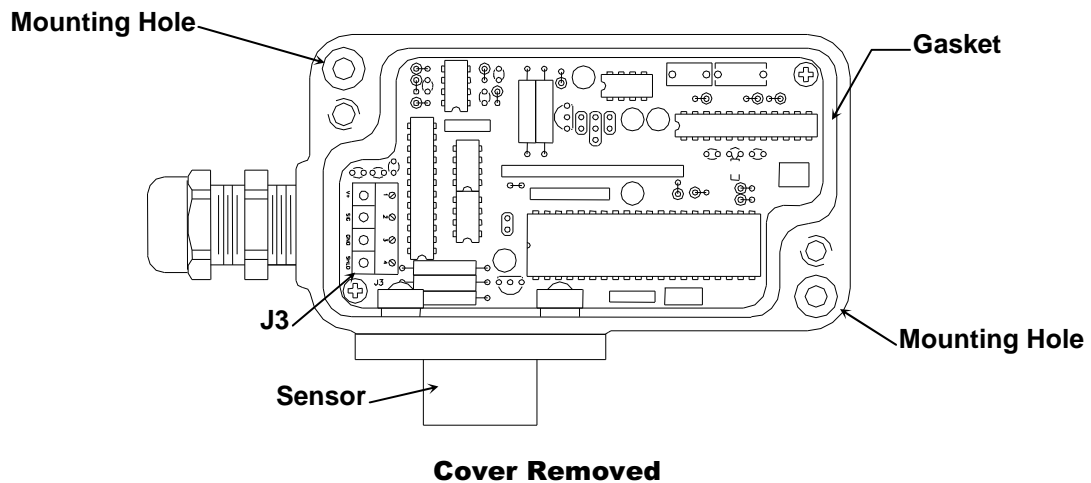
Figure A: SDS – 97D Sensor/Transmitter
