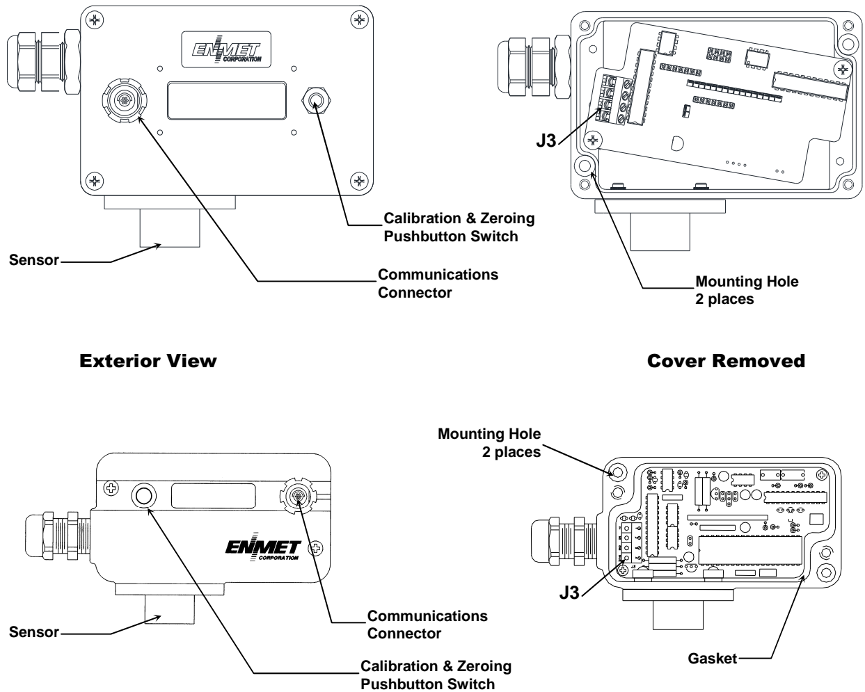
Figure A: SDS – 97D Sensor/Transmitter
