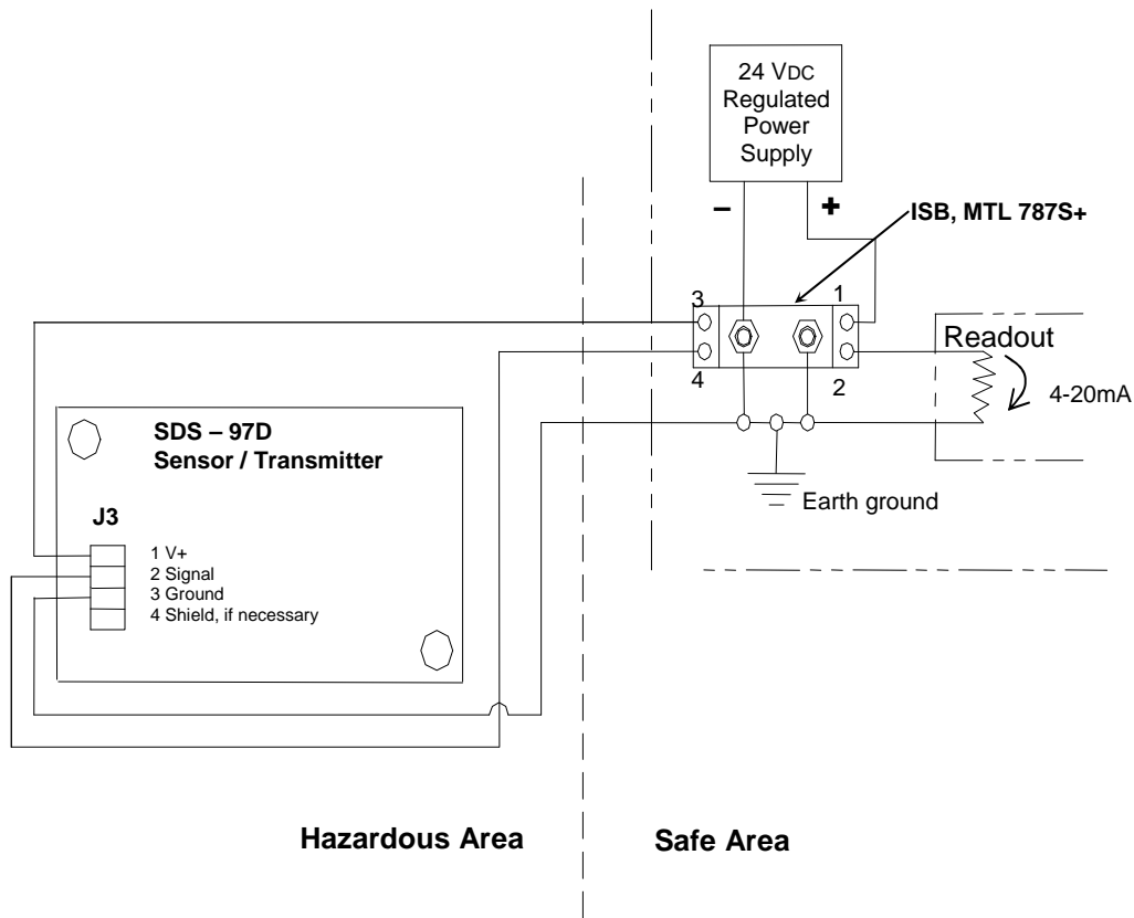
Figure C: Wiring to ISB
