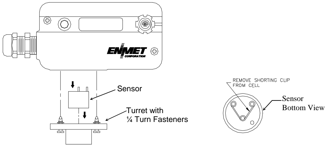
Figure F: SDS – 97D Sensor/Transmitter with Turret and Sensor Removed
