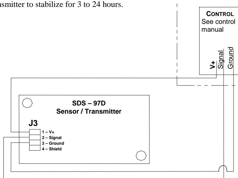
Figure B: Direct Wiring to CONTROL
