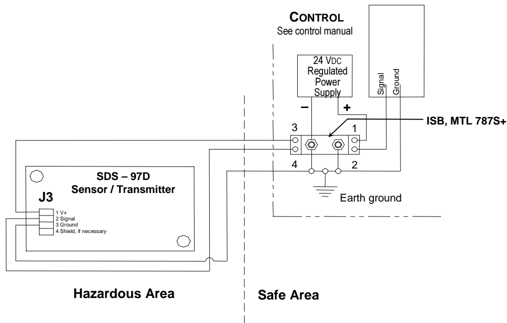
Figure D: Wiring to ISB in CONTROL
