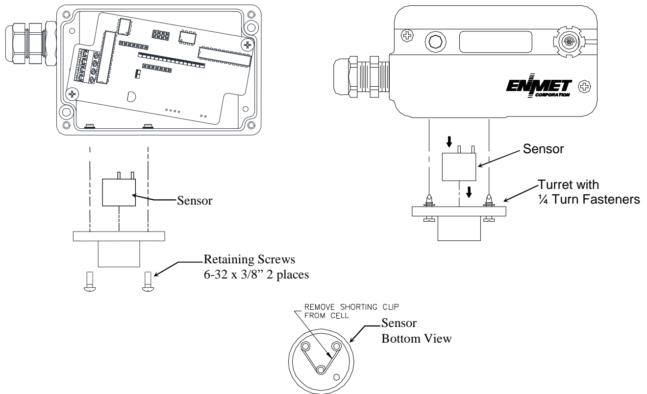
Figure F: SDS – 97D Sensor/Transmitter with Turret and Sensor Removed
