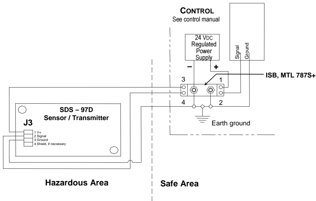
Figure D: Wiring to ISB in CONTROL
