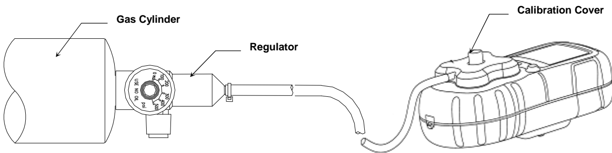
Figure 3: Calibration of RECON/4
