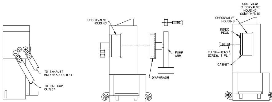
Figure 5: Check Valve Housing Replacement Details
