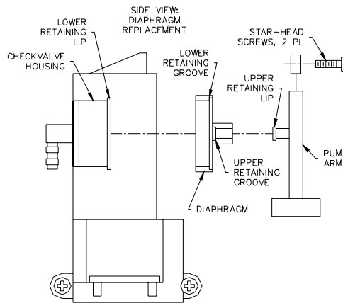
Figure 4: Diaphragm Details
