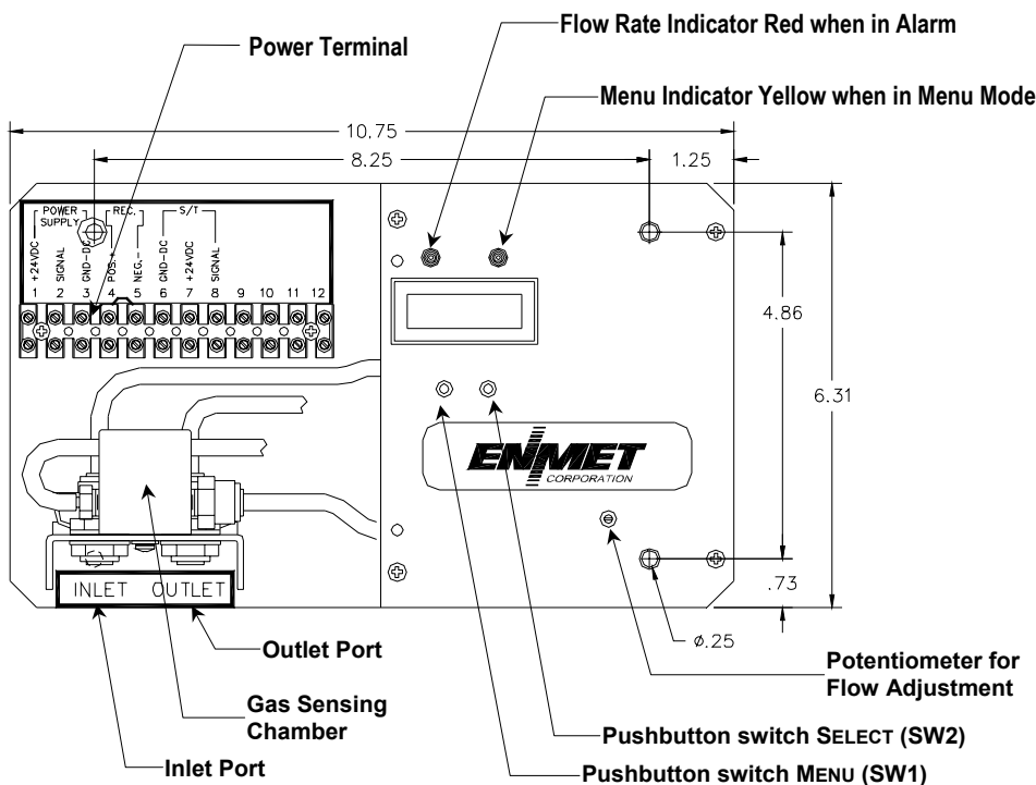
Figure 1: Front View
