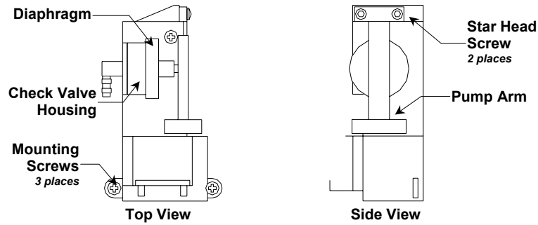
Figure 3: Pump Features
