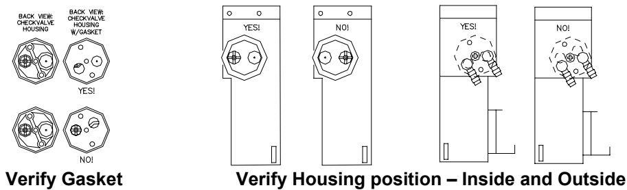
Figure 6: Proper Orientation of Check Valve Housing and Gasket
