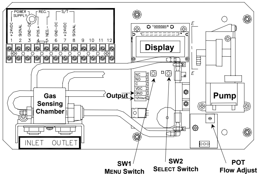
Figure 2: Interior View
