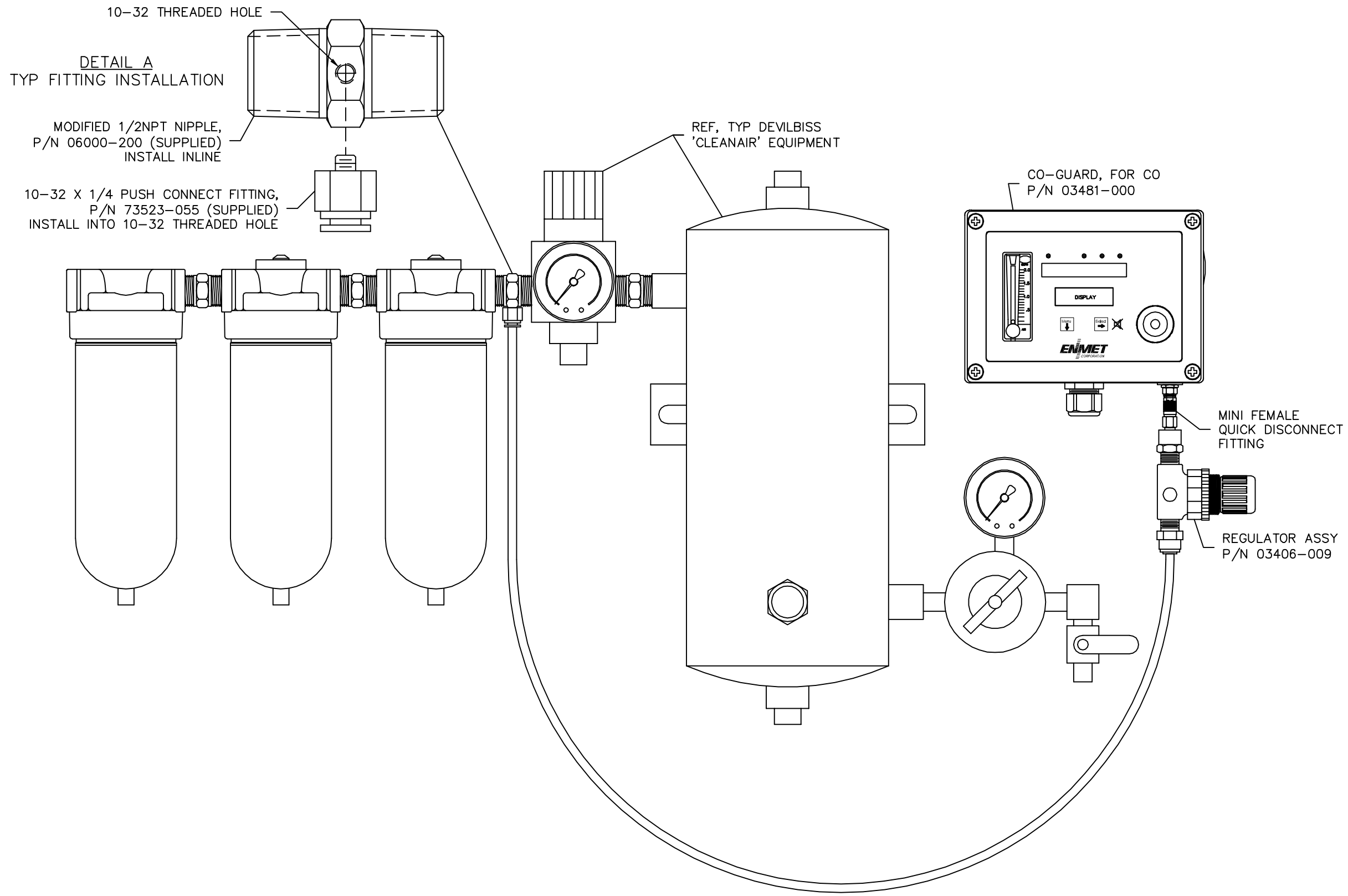
CO-GUARD, FOR CO, DEVILBISS, P/N 03481-021 USE FOR A MANUAL DRAWING
